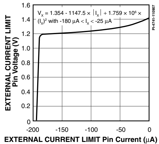
Figure 45. EXTERNAL CURRENT LIMIT Pin Voltage vs. Current.
