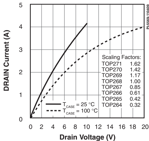
Figure 48. Output Characteristics.
