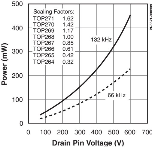
Figure 51. DRAIN Capacitance Power.
