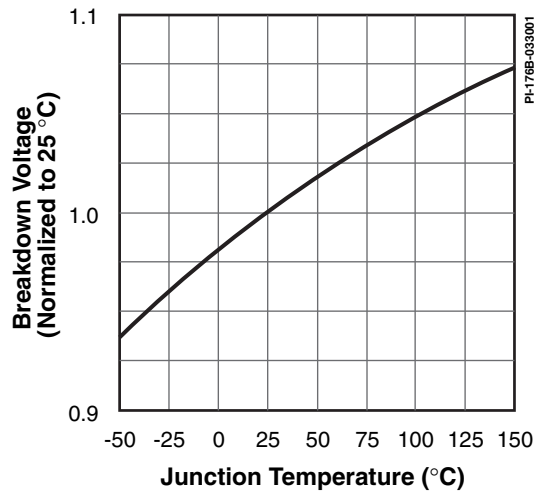
Figure 38. Breakdown Voltage vs. Temperature.
